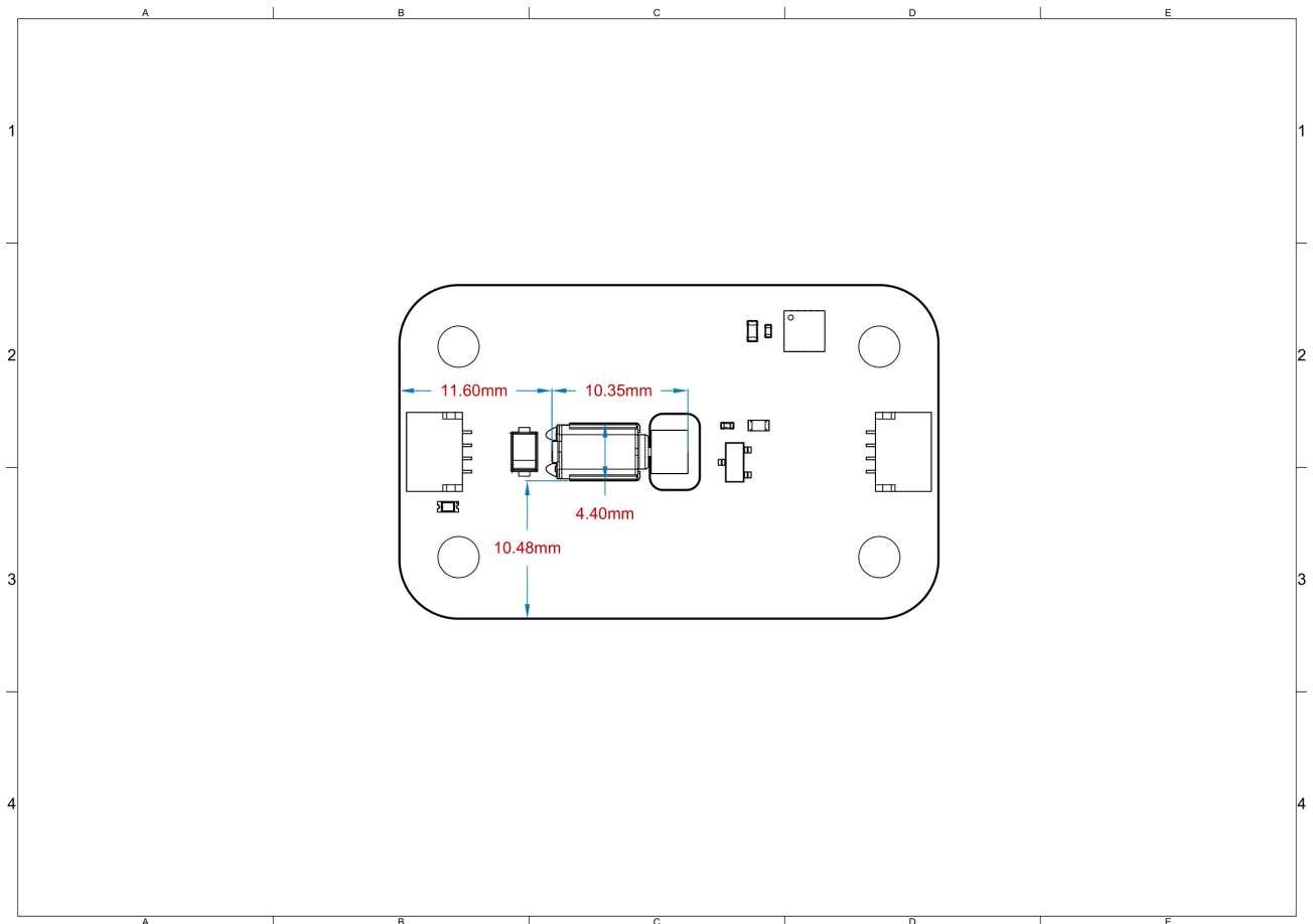
Modulino® Vibro Mechanical Information
