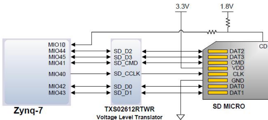
Figure 6-10: SD Card Connection Diagram
