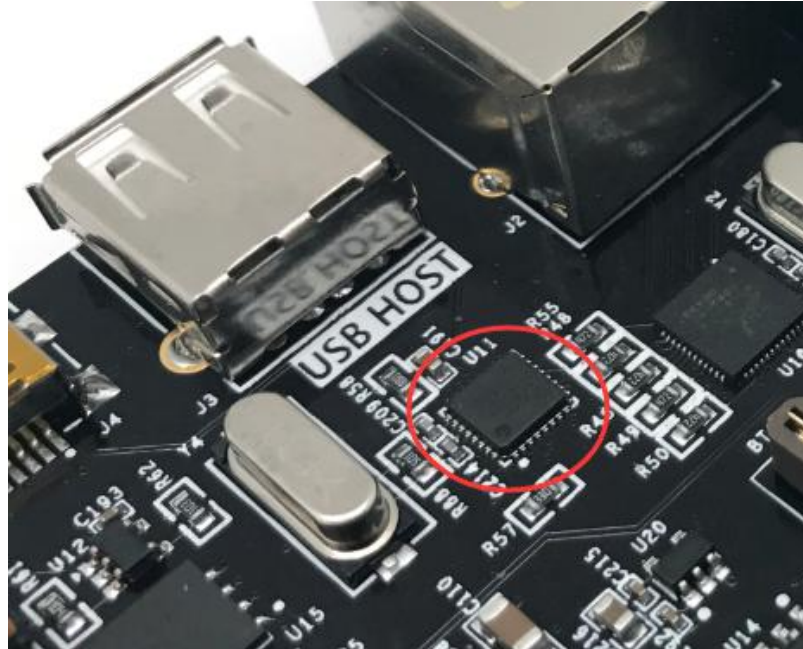
Figure 6-7: The USB3320C chip on the FPGA Board
