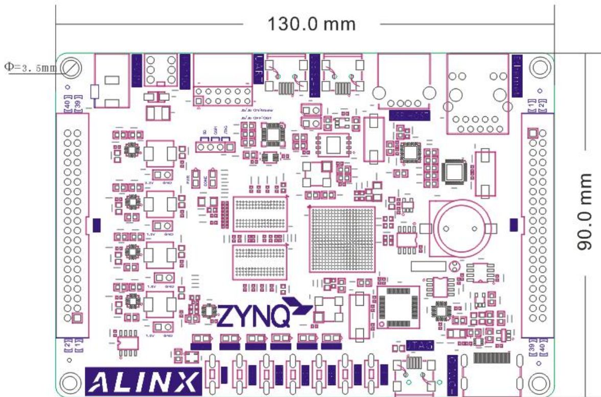
Figure 2-1: FPGA Size Dimension
