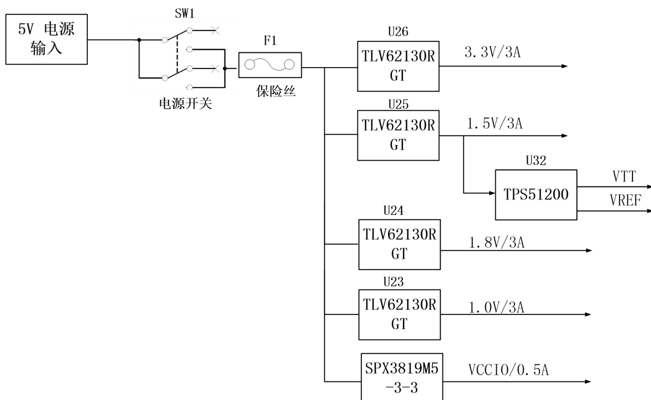
Figure 3-1: Power Supply Schematic
