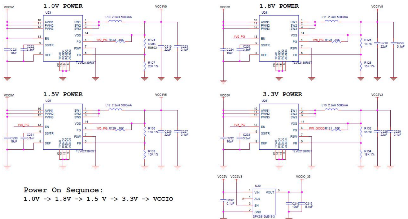
Figure 3-2: Power Supply Circuit
