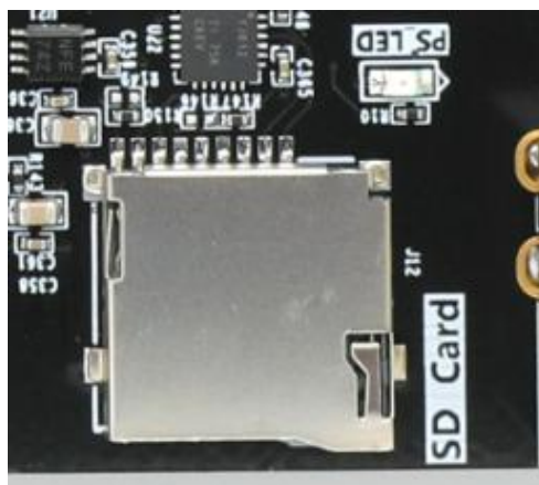
Figure 6-11: SD Card Slot on the FPGA Board
