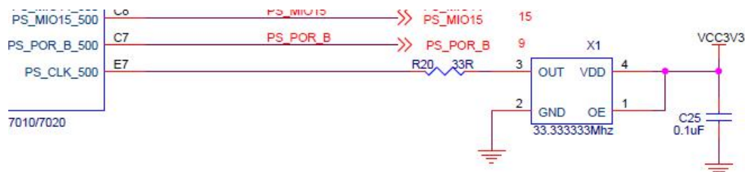
Figure 5-1: Active crystal oscillator to the PS section
