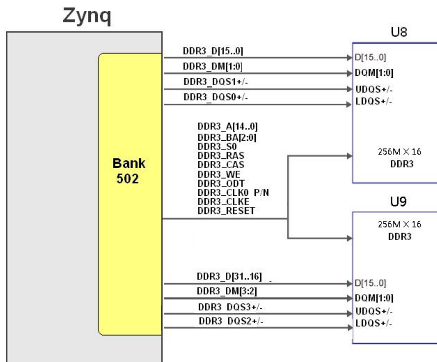
Figure 6-2: The Schematic Part of DDR3 DRAM
