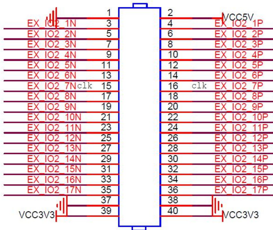
Figure 7-9: Expansion header J10 schematic
