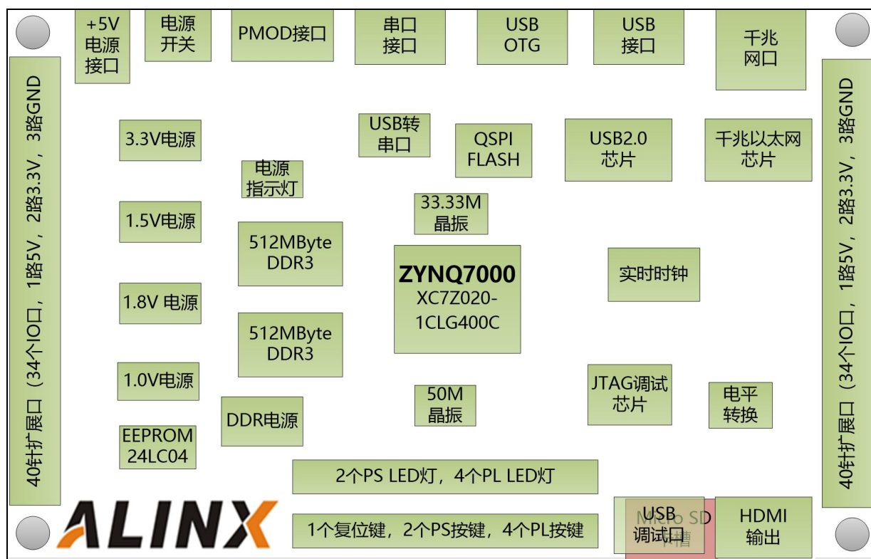
Figure 1-1: The Schematic Diagram of the AX7020
