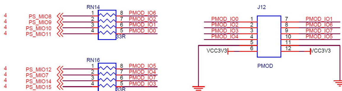
Figure 6-12: PS PMOD connector Schematic
