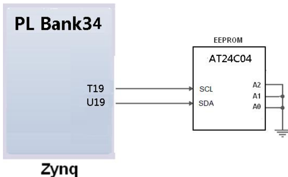
Figure 7-5: EEPROM Schematic
